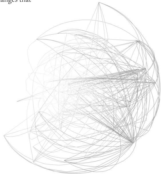
4.4.7 emergent clustering of web pages when Valence is applied to web site usage data
