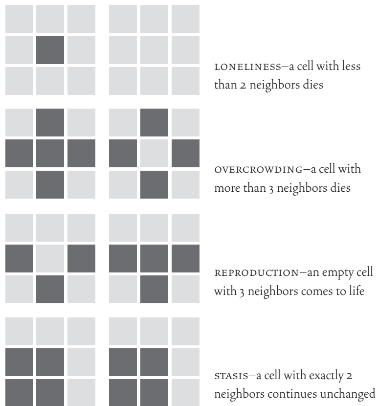
2.1.2 rules for Conway’s Life —in the examples, only the center element is affected by the rule
